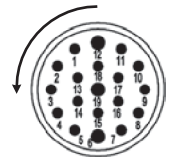
Insert Socket Mating View (counterclockwise orientation)
