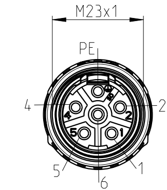
socket face female
