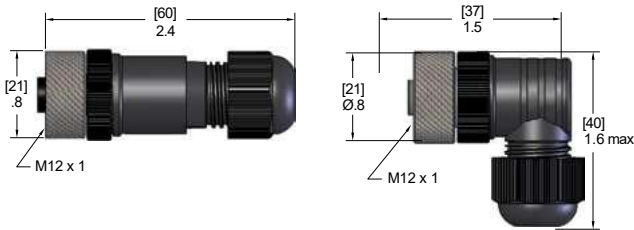
Female Straight
