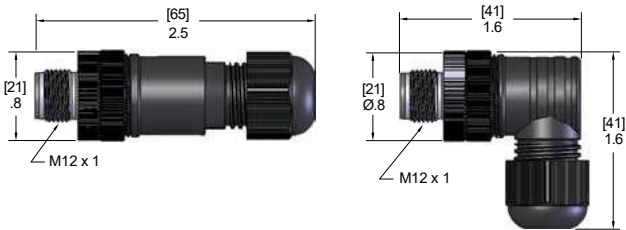
Male Straight
