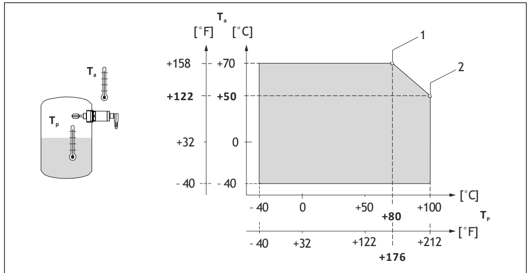
Fig 5 Derating curve: 100 °C (212 °F)
