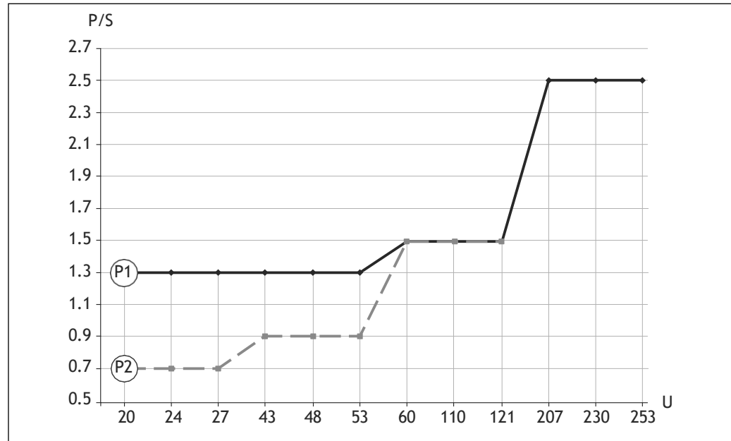
Fig. 1 Minimum rated power of the load
