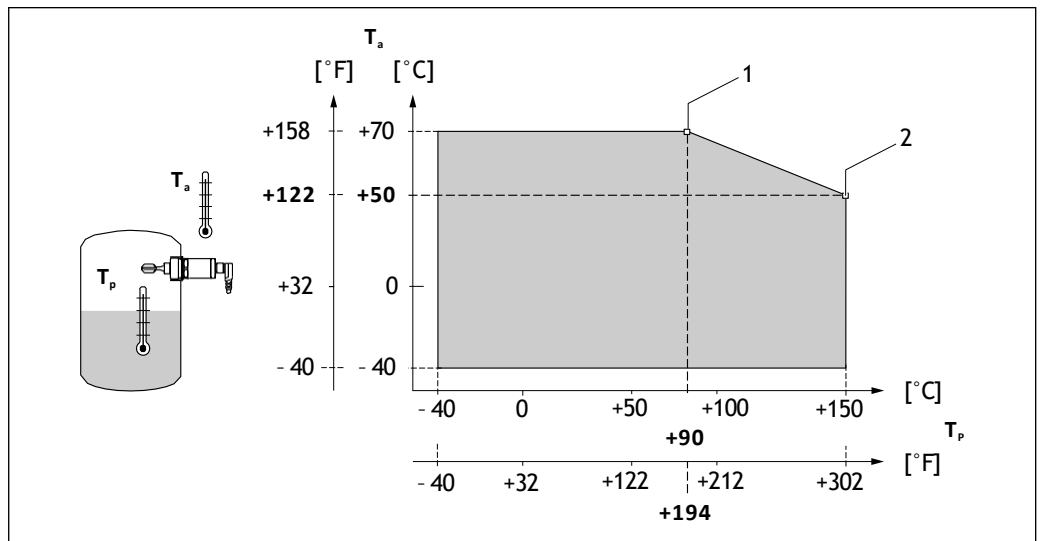
Fig 6 Derating curve: 150 °C (302 °F)
