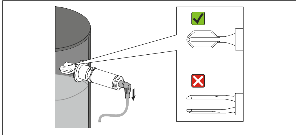
Fig 4 Position of the fork in the case of horizontal installation in a vessel
