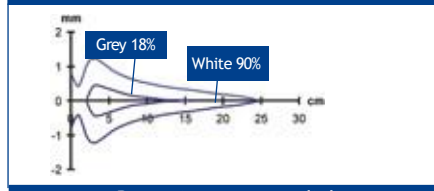
Detection area - radial
