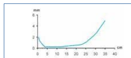
Resolution - axial
