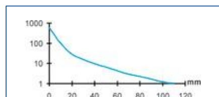
Excess gain - through beam *
