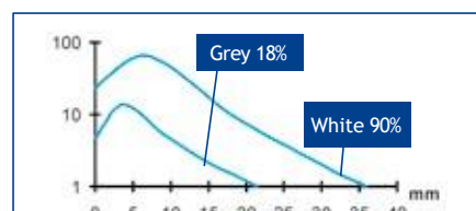
Excess gain - proximity *
