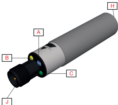
Fig. 2 CA18 Conector
