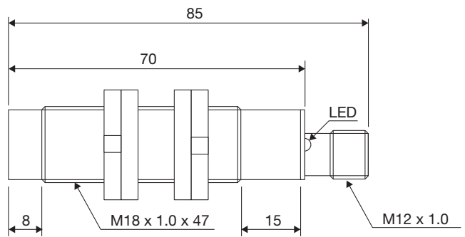
Fig. 9 Conector CA18CAN...M1IO
