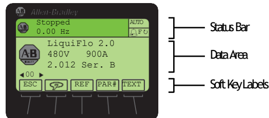
Figure 3 - HIM Display Zones
